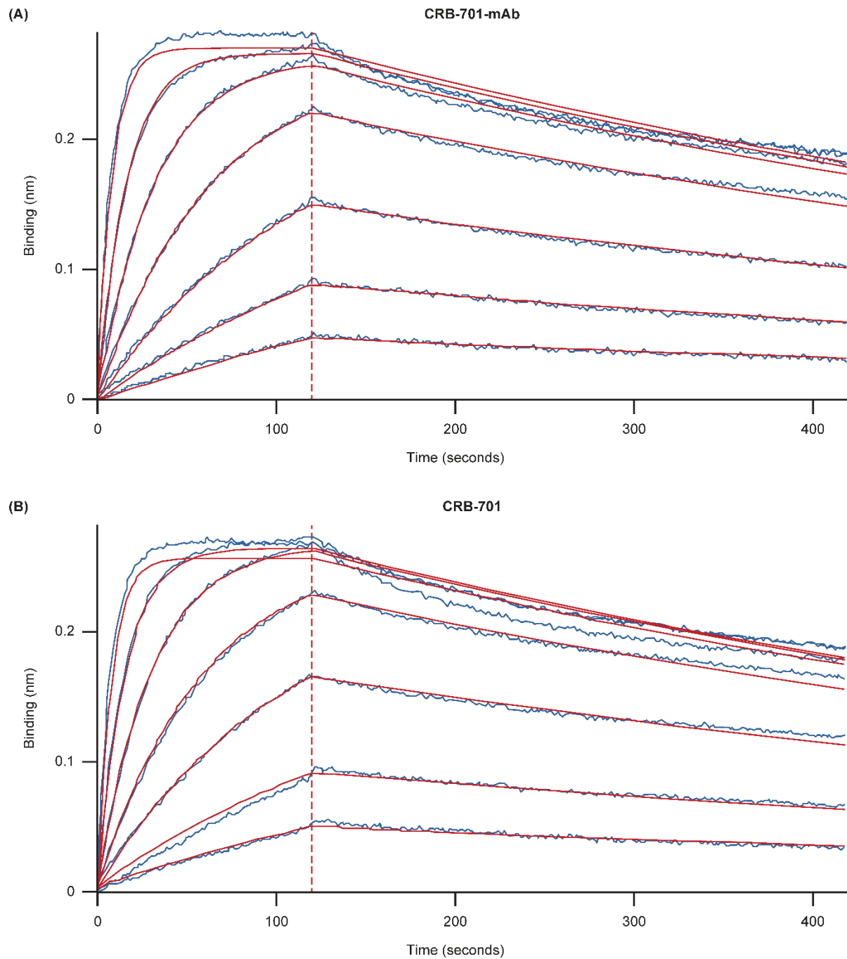
Figure S2. (A) Representative binding curves of interaction between CRB-701-mAb and nectin-4 (fitted to K_d : 2.193 nM; r^2 : 0.9977) and (B) CRB-701 and nectin-4 (fitted to K_d : 2.063 nM; r^2 : 0.9964) as determined by the BLI method.
