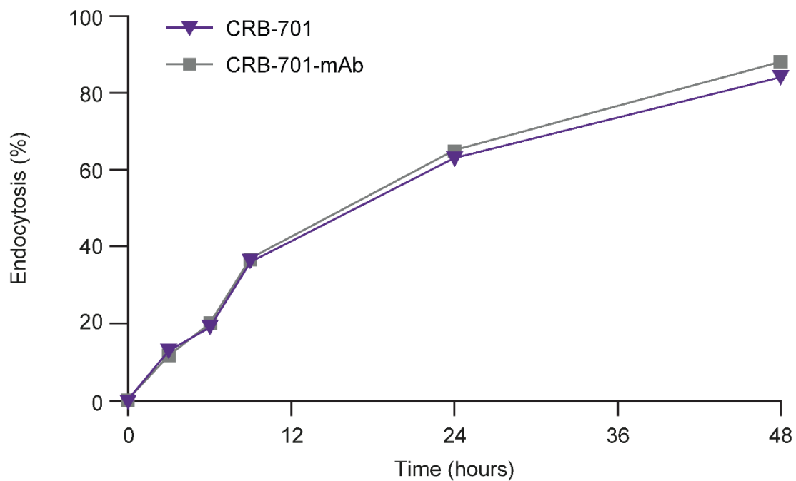
Figure S5. Endocytosis of 2 \mu\text{g/mL} CRB-701 or CRB-701-mAb in PC-3-NECTIN4 cells assessed by flow cytometry. Endocytosis percentages were calculated based on MFI reduction.
