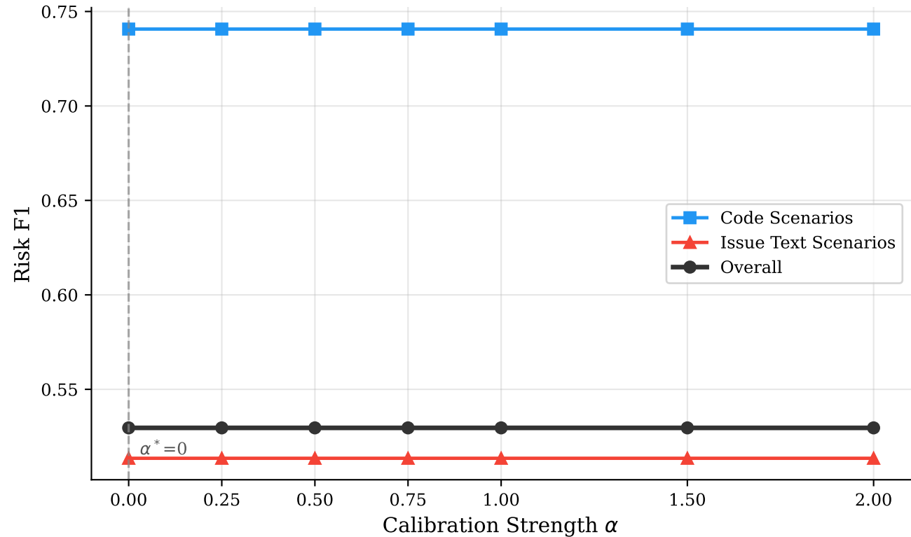
Bayesian Calibration: Risk F1 vs \alpha (qwen-plus)
