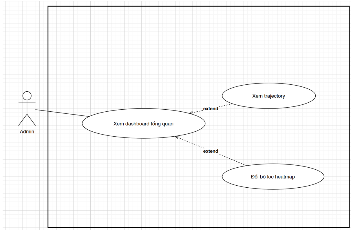
Dashboard.png
