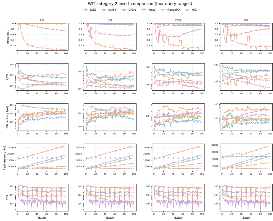
Figure 4: Category-2 insertion workload on WIT.
