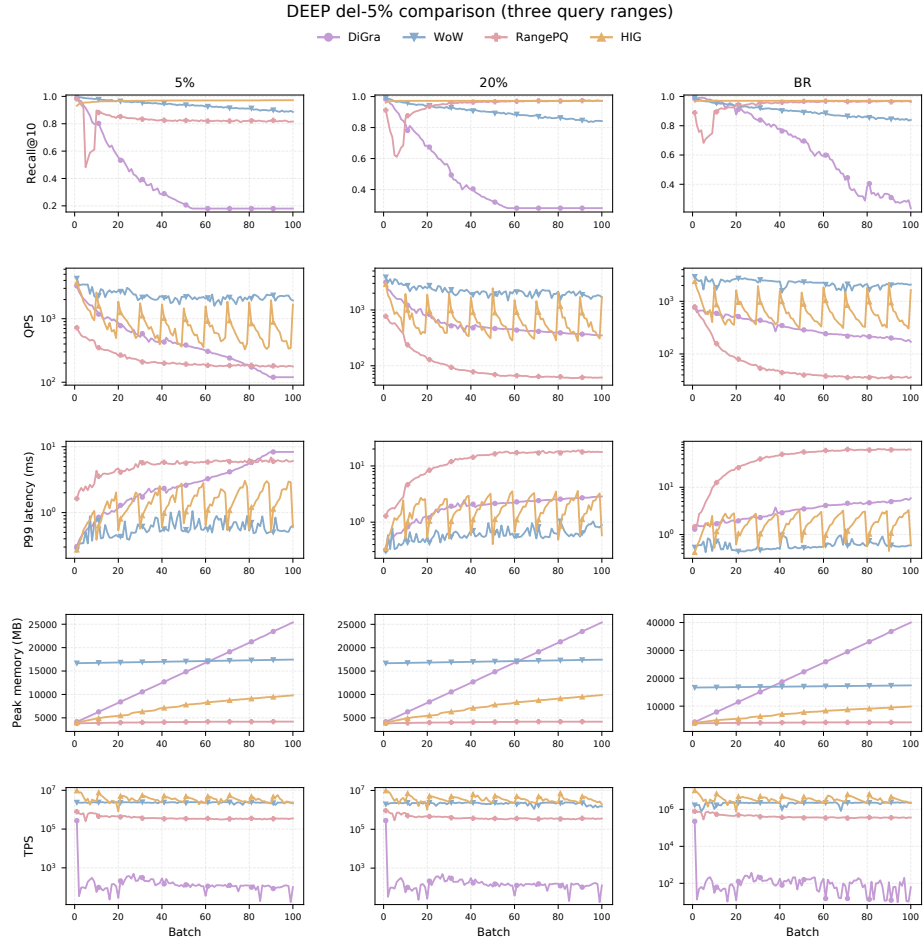
Figure 6: Deletion workload under del5% on DEEP.
