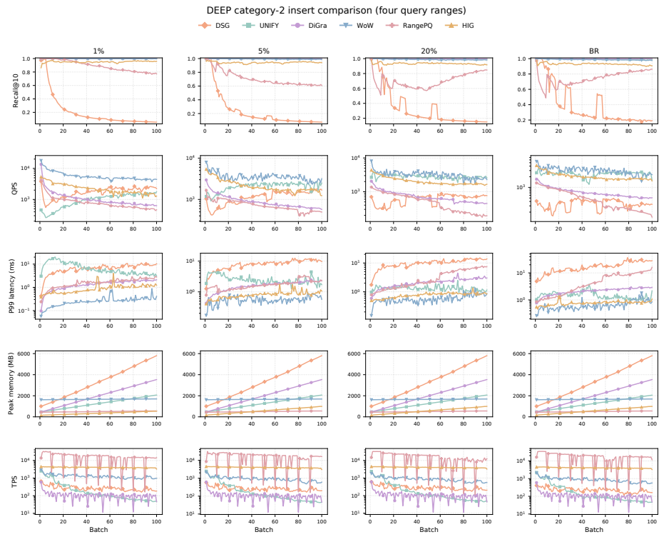
Figure 3: Category-2 insertion workload on DEEP.
