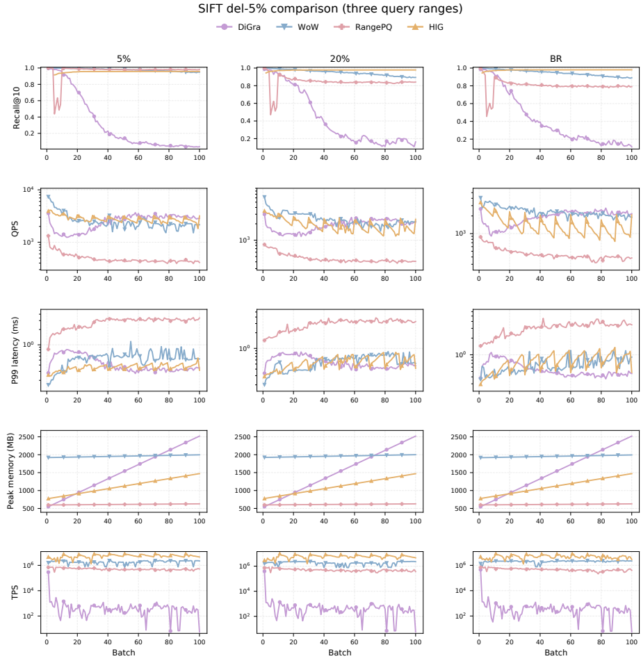
Figure 5: Deletion workload under del5% on SIFT.
