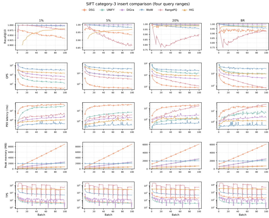
Figure 1: Category-3 insertion workload on SIFT.
