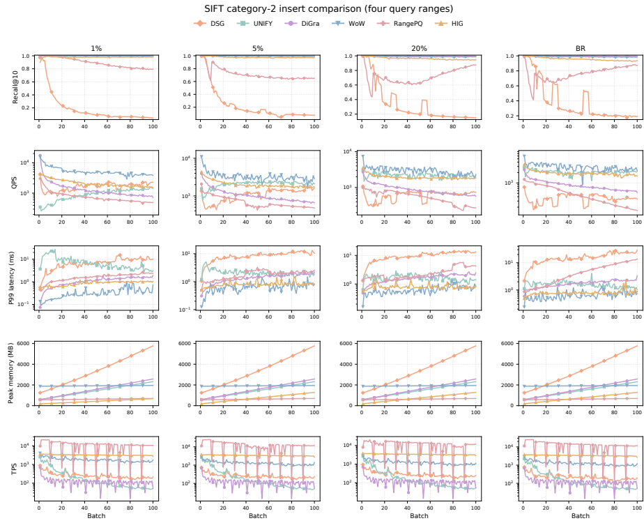
Figure 2: Category-2 insertion workload on SIFT.
