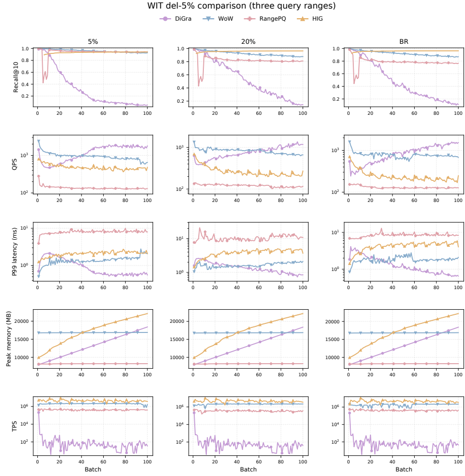
Figure 7: Deletion workload under del5% on WIT.
