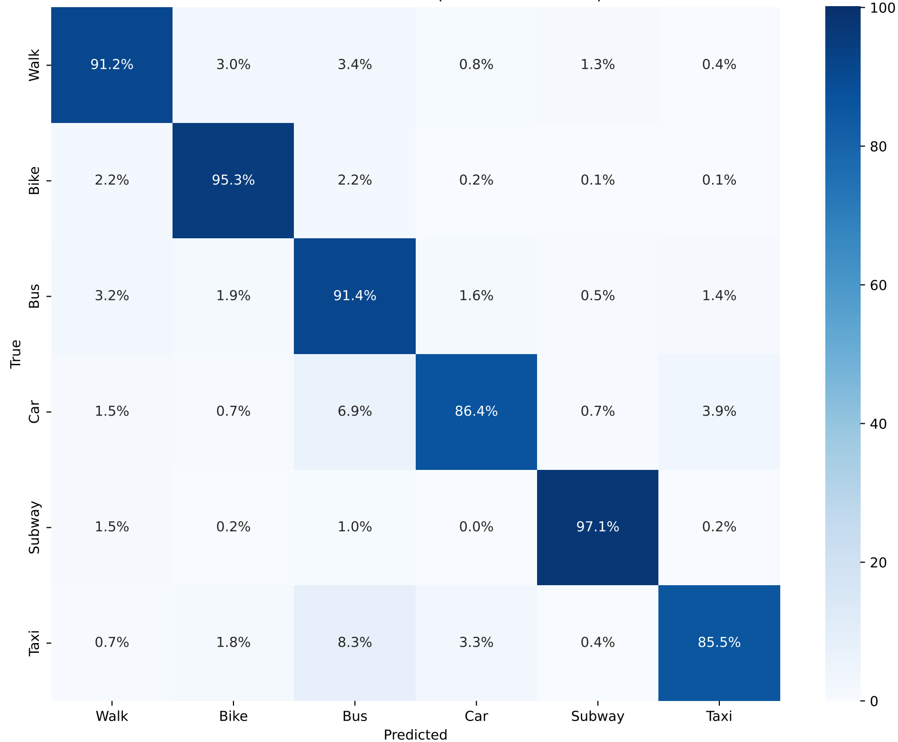
6-Class Confusion Matrix (Row-Normalized %)
