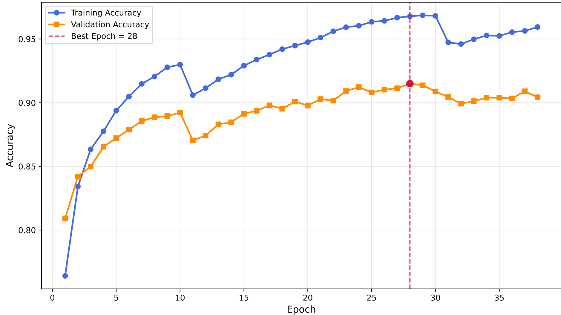
Training and Validation Accuracy over Epochs
