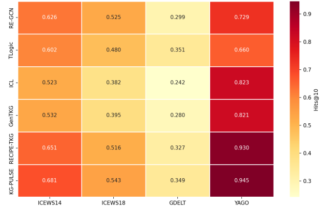
Hits@10 Performance Across Datasets and Models
