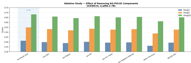
Figure 11: Ablation: Hits@10 on ICEWS14 when each component is removed. All five components contribute positively.
