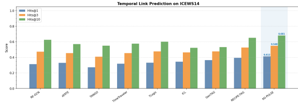
Figure 2: Hits@1/3/10 on ICEWS14 [16] across all models. KG-PULSE achieves the highest scores on all three metrics.
