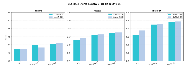
Figure 9: LLaMA-2 vs. LLaMA-3 backbone comparison on ICEWS14.
