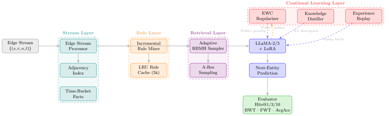
Figure 1: KG-Pulse System Architecture. Solid grey arrows show the forward data path from raw edge stream to prediction and evaluation. Dashed blue arrows carry gradient-level feedback from the Continual Learning Layer to the LLM Core. The dashed orange arrow shows the Fisher information update used by EWC. Four colour-coded subsystem layers are highlighted.
