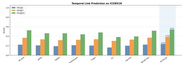
Figure 3: Hits@1/3/10 on ICEWS18 [16] across all models. KG-PULSE yields the largest relative gain (+6.7% H@1) due to the large entity vocabulary (23,033 entities) where the streaming incremental rule miner is most efficient.
