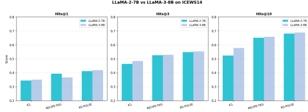
Figure 9: LLaMA-2 vs. LLaMA-3 backbone comparison on ICEWS14.
