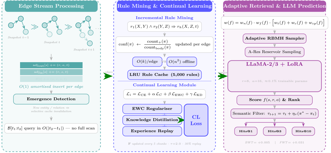
Figure 1: Overview of the KG-Pulse Framework. Left: The Edge Stream Processor ingests a continuous stream of timestamped facts, maintaining O(1) adjacency indices ( \text{adj}_{\text{out}} , \text{adj}_{\text{in}} , \mathcal{B}[t] ) and issuing emergence events for unseen entities or relations. Middle (top): The Incremental Rule Miner updates rule confidences in O(k) per edge (vs. O(n^2) offline), storing active rules in an LRU cache of 5,000 entries. Middle (bottom): The Continual Learning Module combines EWC, Knowledge Distillation, and Experience Replay into a single CL loss, achieving \text{BWT} = +0.005 (near-zero forgetting). Right: The Adaptive RBMH Sampler retrieves evidence via A-Res reservoir sampling; LLaMA-2/3 + LoRA scores candidate entities; an online semantic filter (threshold \tau_t ) prunes implausible outputs before ranking to Hits@1/3/10.
