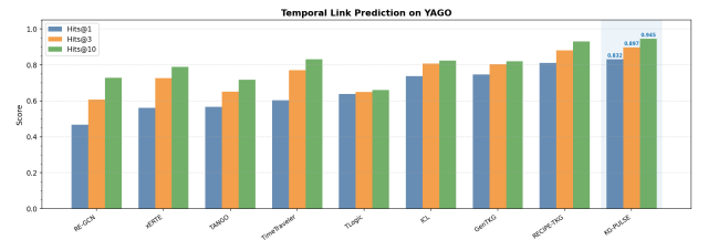
Figure 5: Hits@1/3/10 on YAGO [18] across all models. Gains are more modest (+2.6% H@1) due to coarse annual granularity and a small relation vocabulary (24 types), but the continual learning module prevents the regression that naive fine-tuning causes.
