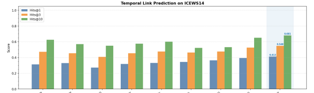
Figure 2: Hits@1/3/10 on ICEWS14 [16] across all models. KG-PULSE achieves the highest scores on all three metrics.
