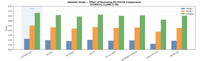
Figure 11: Ablation: Hits@10 on ICEWS14 when each component is removed. All five components contribute positively.
