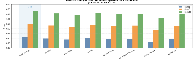
Figure 8: Ablation study — component removal effects on ICEWS14.
