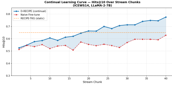
Figure 4: Hits@10 over stream chunks (ICEWS14). D-RECIPE maintains and improves performance; Naive Fine-tune degrades.
