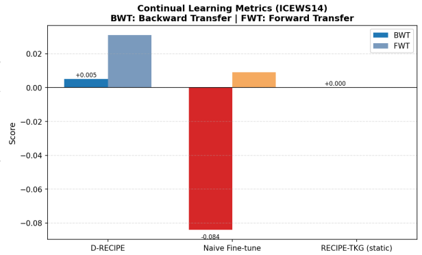
Figure 5: BWT and FWT comparison. Positive BWT in D-RECIPE indicates that past periods benefit from continual updates.
