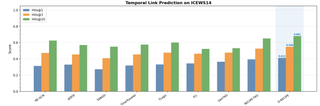
Figure 2: Hits@1/3/10 on ICEWS14 — D-RECIPE vs. all baselines.
