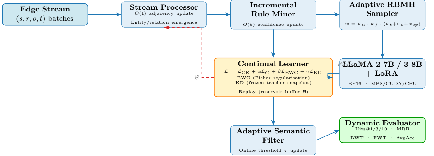
Figure 1: D-Recipe Architecture. Edges arrive as a stream and are ingested by the Stream Processor in O(1) time. The Incremental Rule Miner updates temporal rule confidences in O(k) per edge. The Adaptive RBMH Sampler selects historical context using a composite weight. The Continual Learner optimises the LoRA-adapted LLM with a multi-term loss and experience replay (red dashed loop). The Adaptive Semantic Filter post-processes predictions at inference time.
