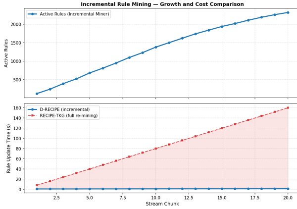
Figure 7: Rule growth and mining time. Incremental mining (D-RECIPE) has near-constant cost vs. full re-mining (RECIPE-TKG), which grows linearly with stream length.
