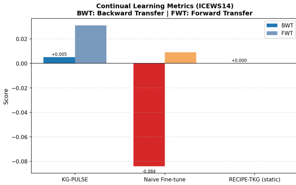
Figure 5: BWT and FWT comparison. PULSE’s near-zero BWT confirms that EWC + KD + Replay successfully prevents forgetting. Positive FWT demonstrates genuine forward knowledge transfer.
