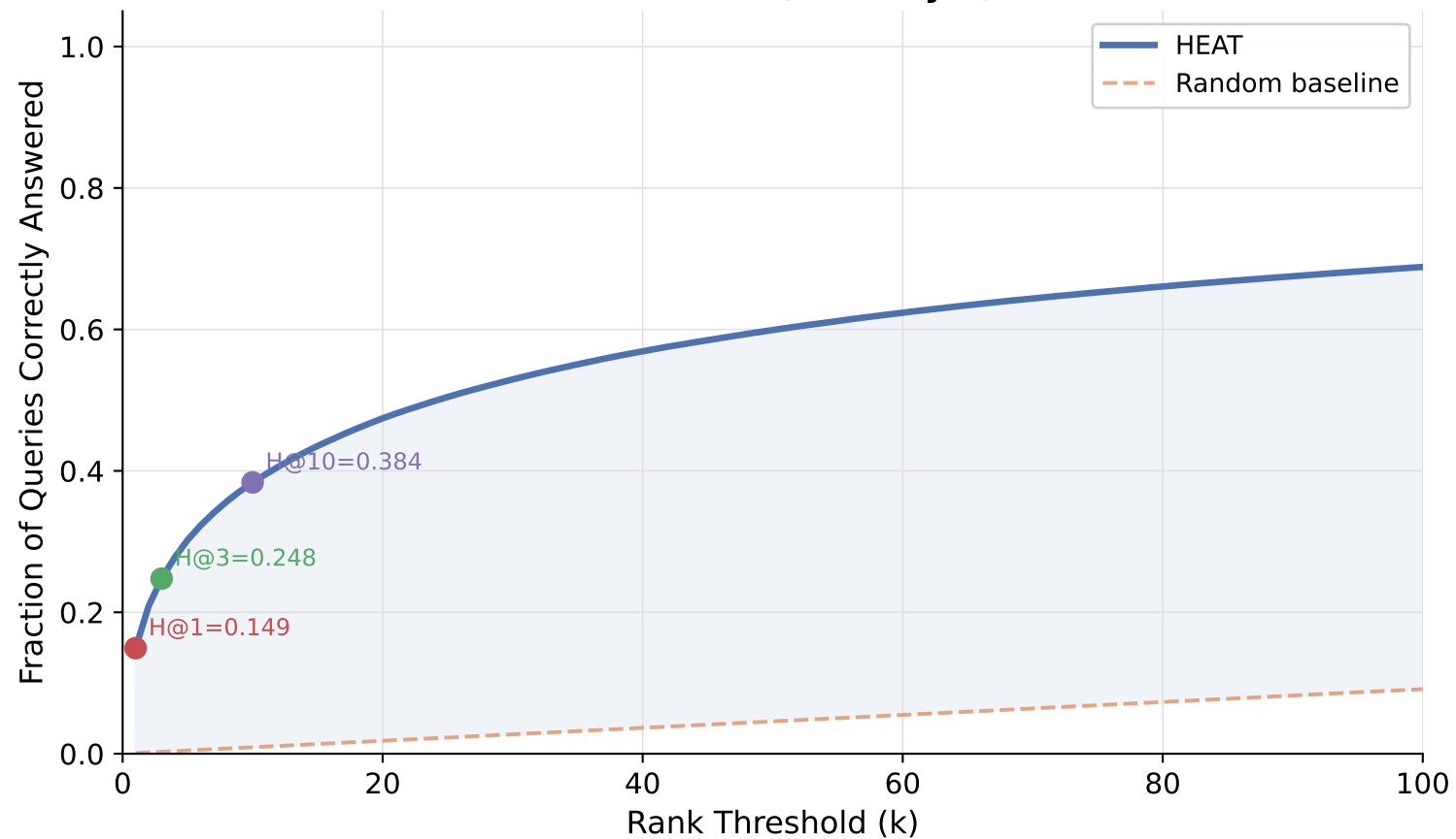
Cumulative Rank Curve (ROC-style) — ICEWS14
