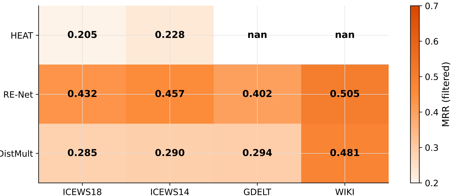
MRR Comparison Heatmap — HEAT vs. Baselines
