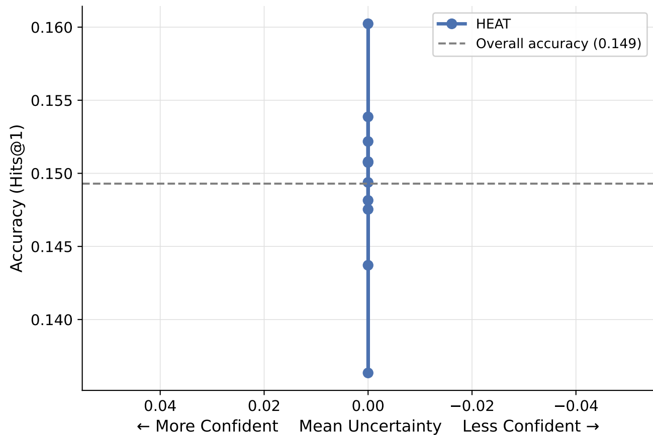
Calibration Plot — ICEWS14
