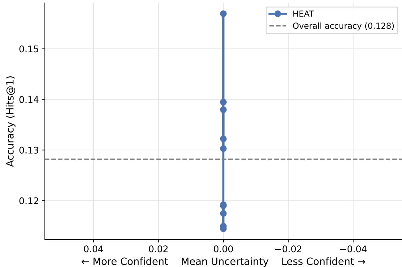
Calibration Plot — ICEWS18
