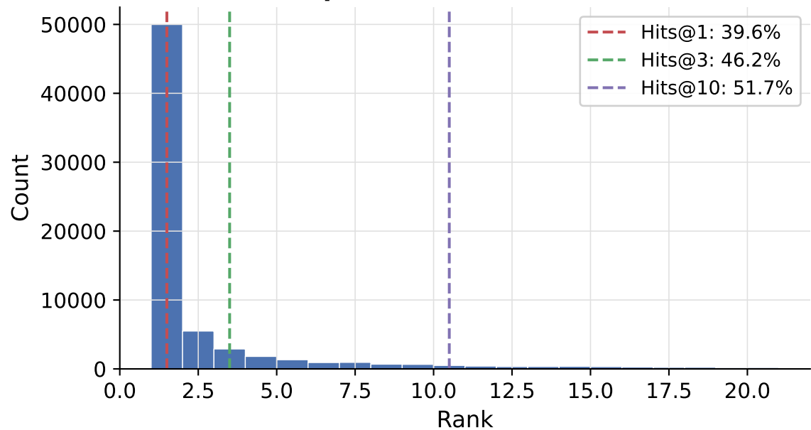
Top-20 Rank Distribution
