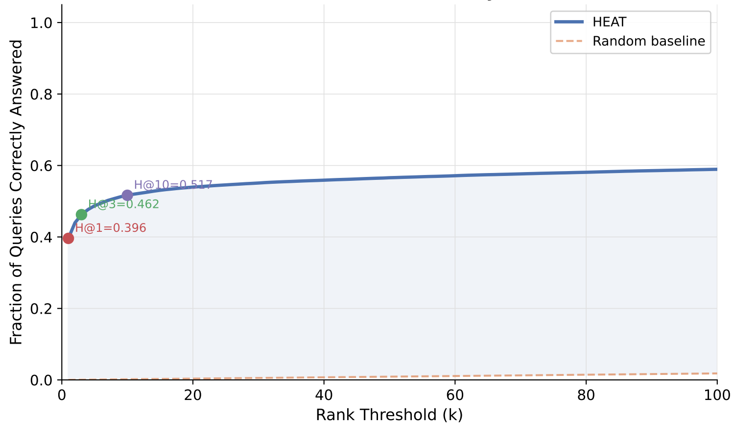
Cumulative Rank Curve (ROC-style) — WIKI
