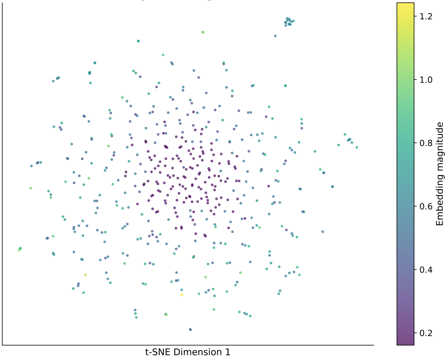
t-SNE of Entity Embeddings — WIKI (n=500)
