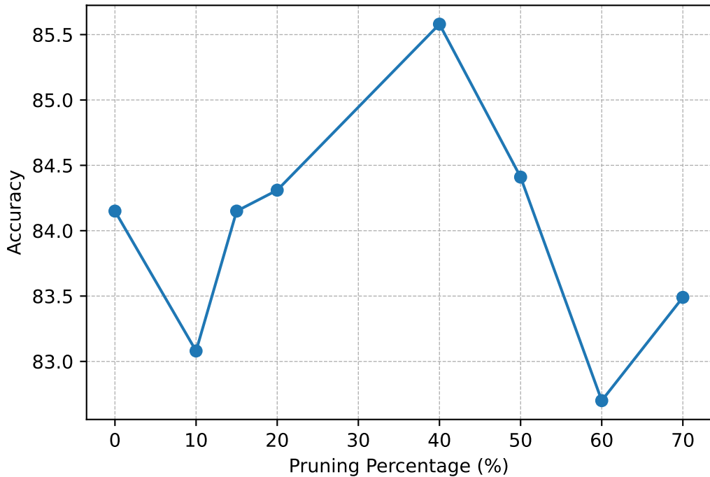
Pruning Percentage vs. Accuracy
