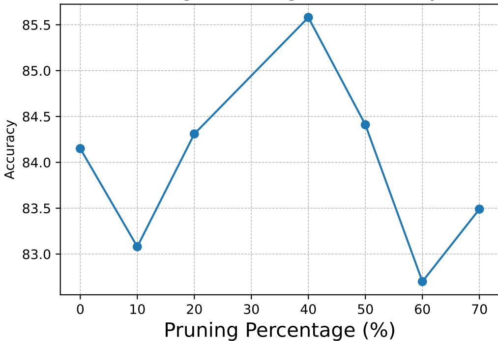
Pruning Percentage vs. Accuracy
