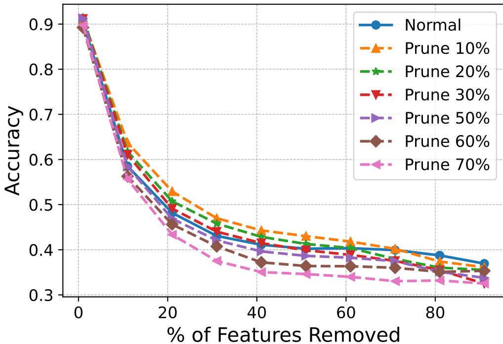
Faithfulness
