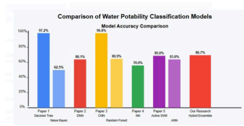
Fig. 3. comparison of water potability classification models.
