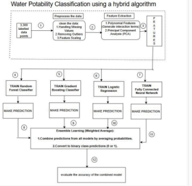
Fig. 1. The hybrid approach data flow is: (1) 3,300 labeled points are given as input. (2) Data is preprocessed to complete missing values, drop outliers, and scale the features. (3) Features are generated via polynomial feature generation (interaction terms) and Principal Component Analysis (PCA). (4) Training is done for a Random Forest Classifier as the first model. (5) Training is performed for a Gradient Boosting Classifier as the second model. (6) A Logistic Regression model is trained as the third model. (7) A Fully Connected Neural Network (FCNN) is trained as the fourth model. (8-11) All the trained models are employed to predict on the test data. The prediction of all the models is merged using a weighted average method by averaging probabilities and transforming them into binary class predictions (0 or 1). (12) Last but not least, the joint model is tested for correctness to verify how well it operates.
