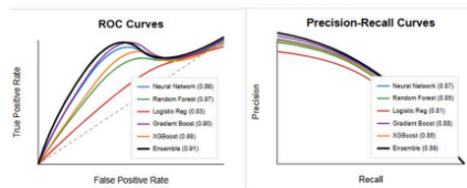
Fig. 10. ROC Curves and Precision-Recall Curves
