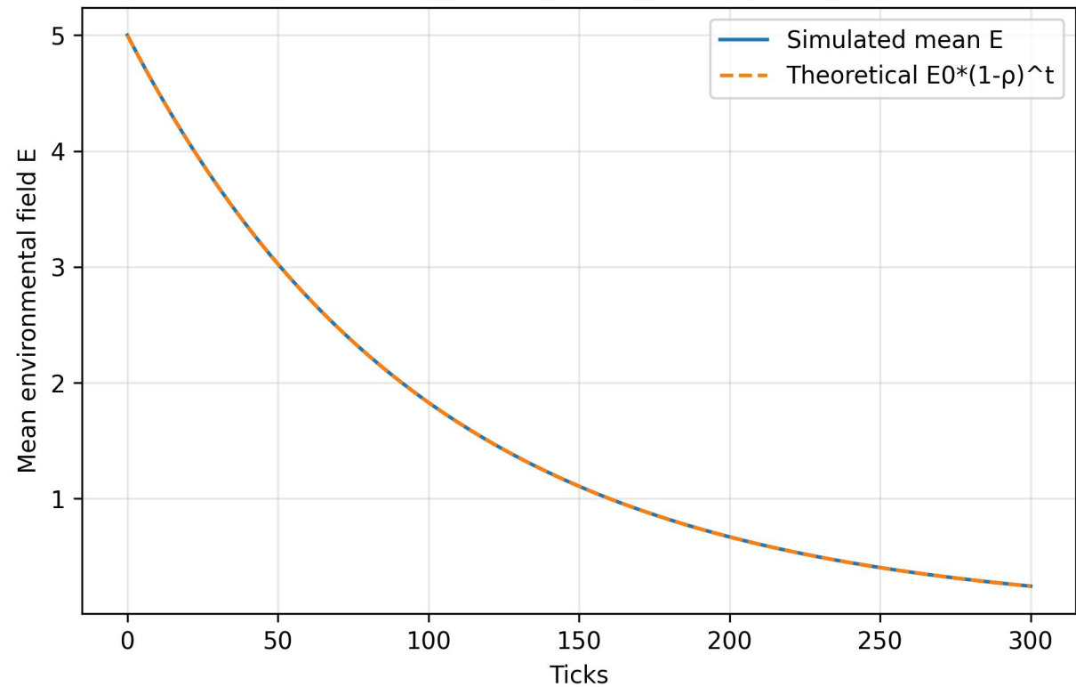
V2 Energy decay test ( \rho=0.01 , D=0 )
