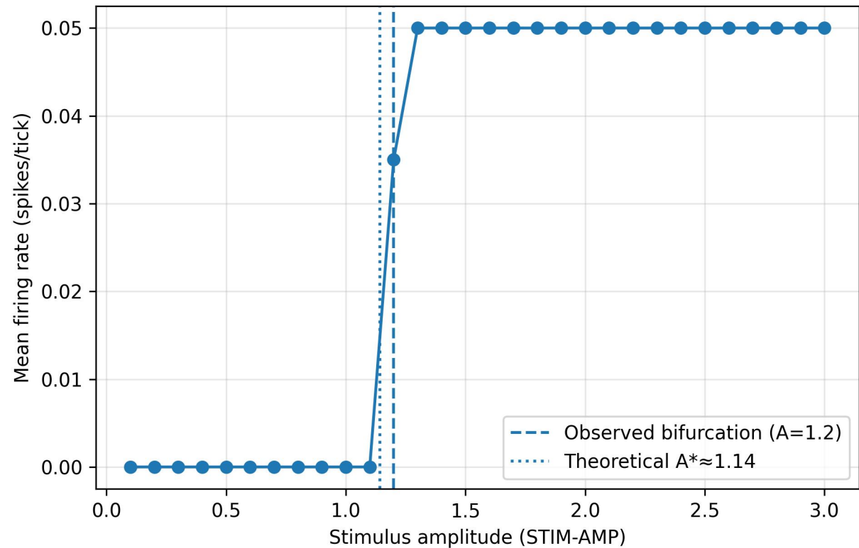
M1 Threshold bifurcation (single neuron)
