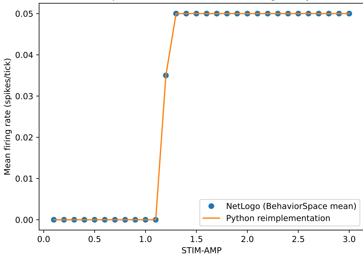
Cross-implementation check (M1): NetLogo vs Python
