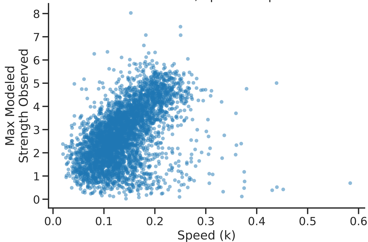
GCN4: Exponential Fit Pearson r=0.49 , Spearman \rho=0.54
