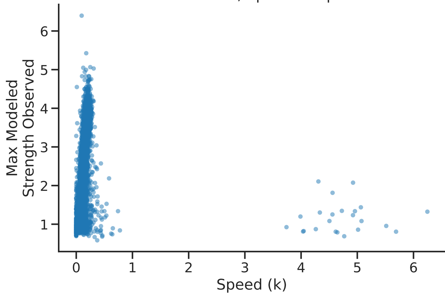
GCN4: Exponential Fit Pearson r=0.02 , Spearman \rho=0.61
