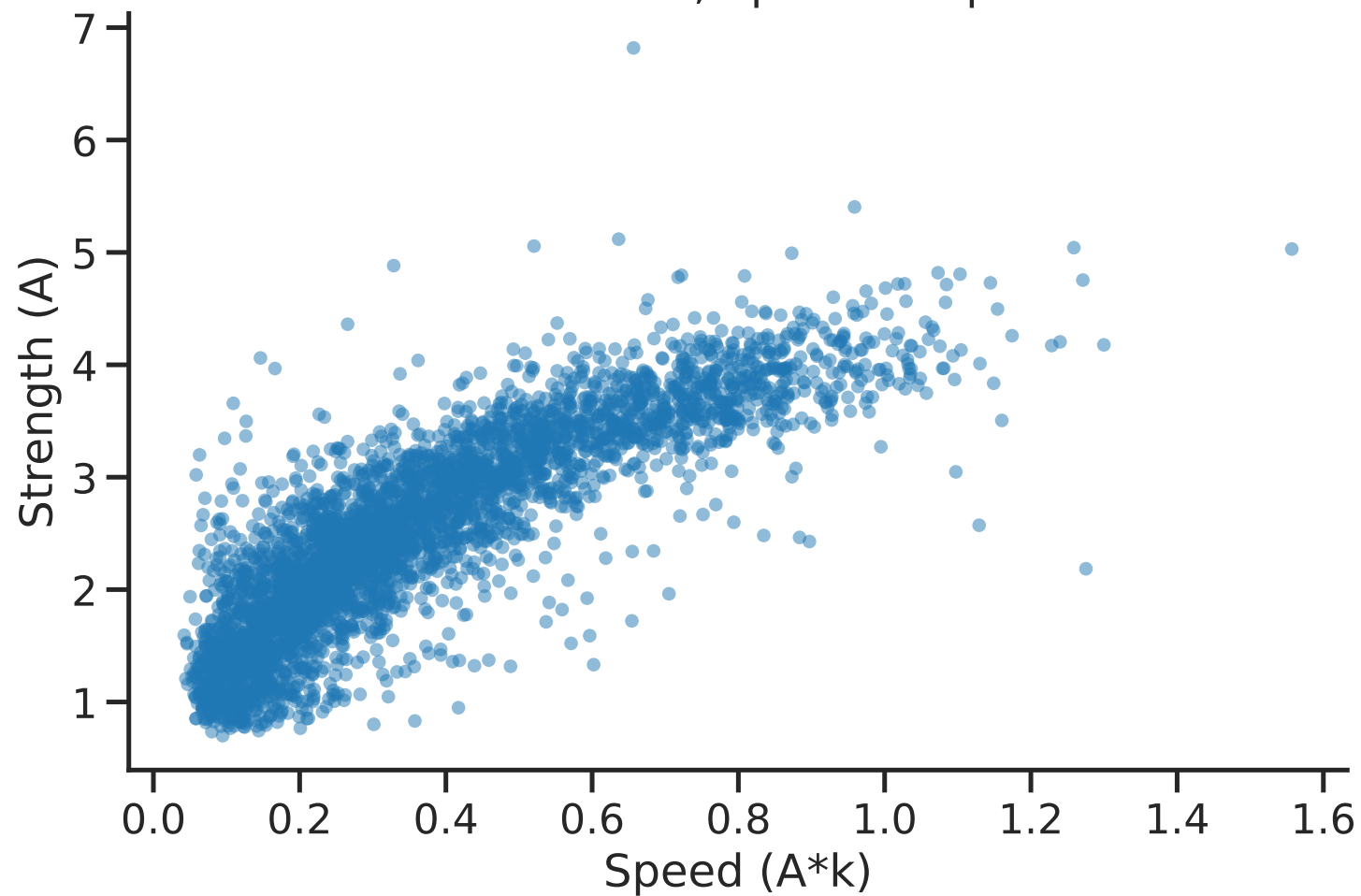
GCN4: Exponential Fit Pearson r=0.85 , Spearman \rho=0.88
