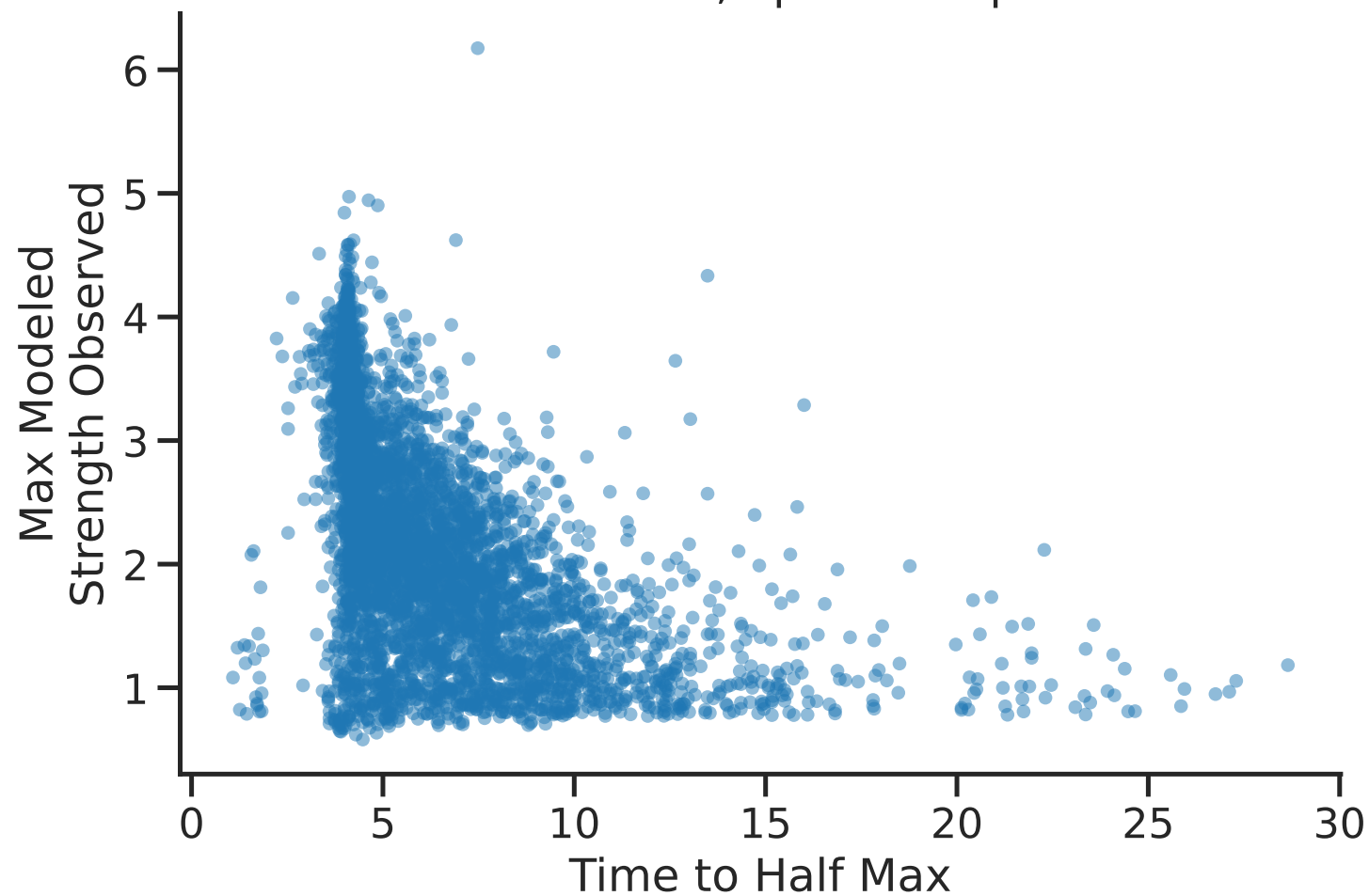
GCN4: Logistic Fit Pearson r=-0.52 , Spearman \rho=-0.62
