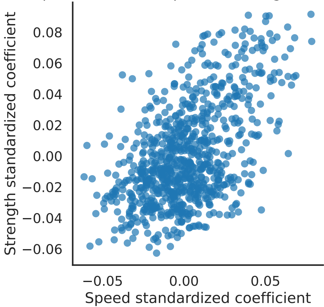
One-hot sequence features: speed vs strength (Linear regression)
