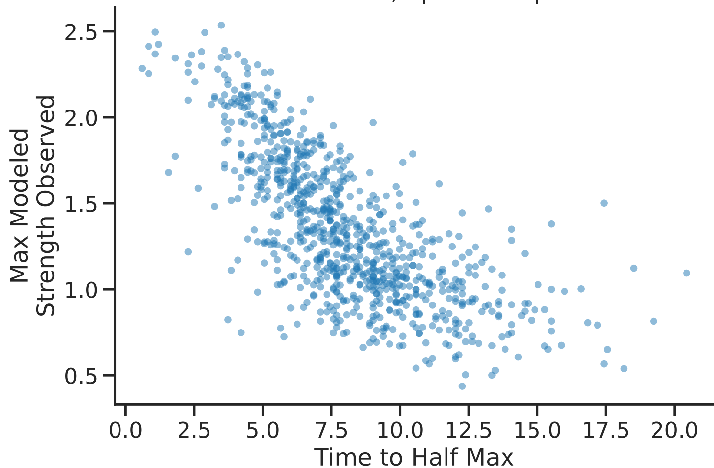
ChopTFs: Exponential Fit Pearson r=-0.72 , Spearman \rho=-0.74
