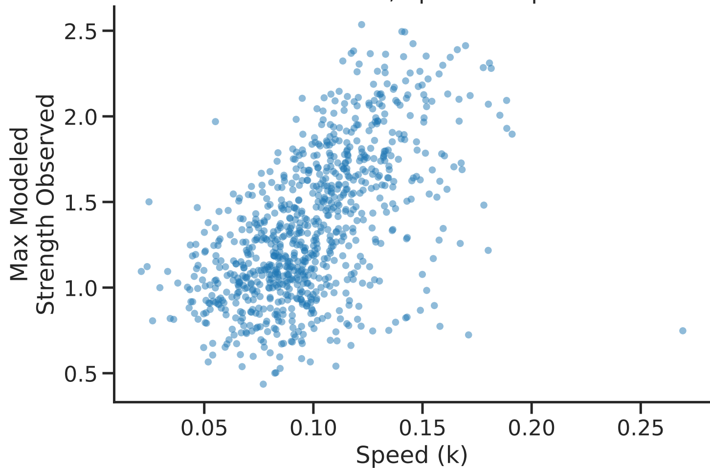
ChopTFs: Exponential Fit Pearson r=0.57 , Spearman \rho=0.59
