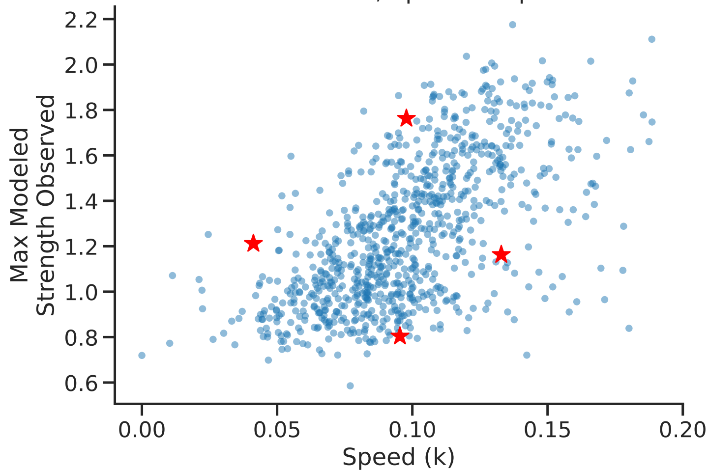
ChopTFs: Exponential Fit Pearson r=0.60 , Spearman \rho=0.63
