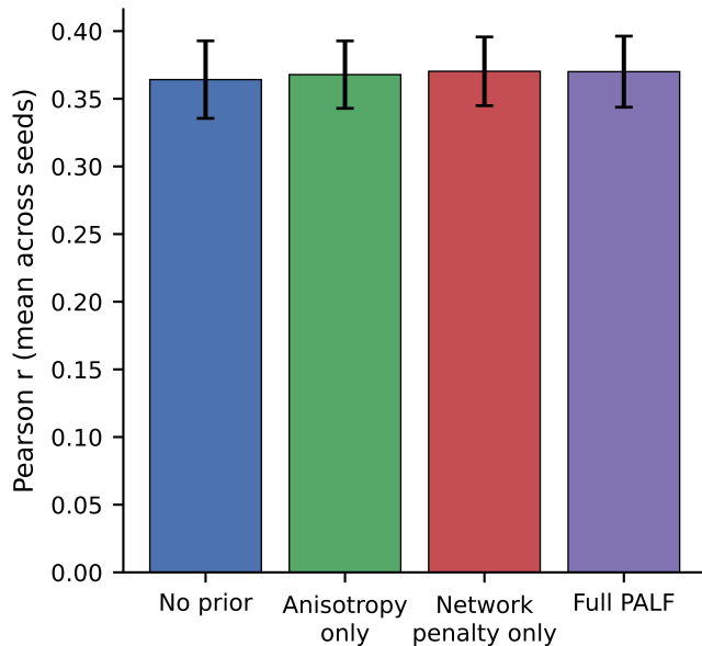
Fluid Intelligence
