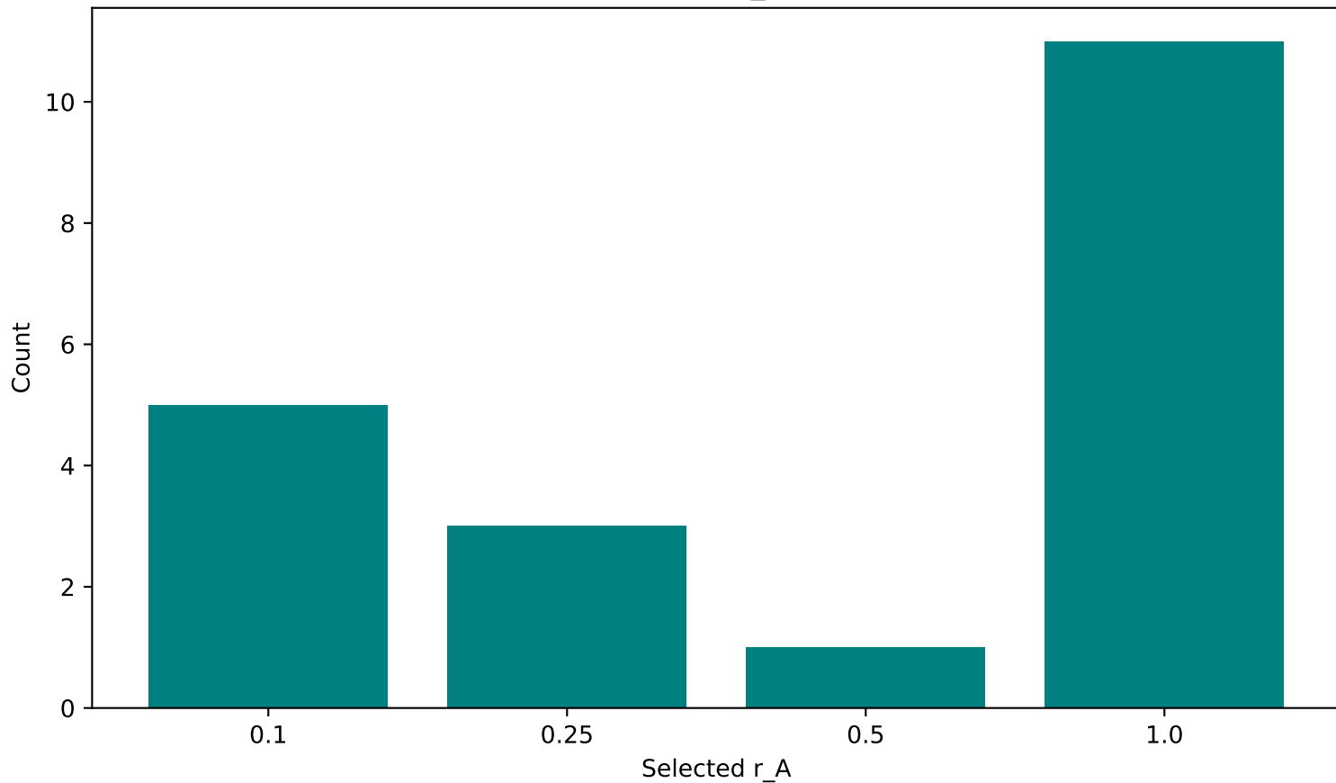
Working Memory: PALF-MPR r_A Selection Distribution
