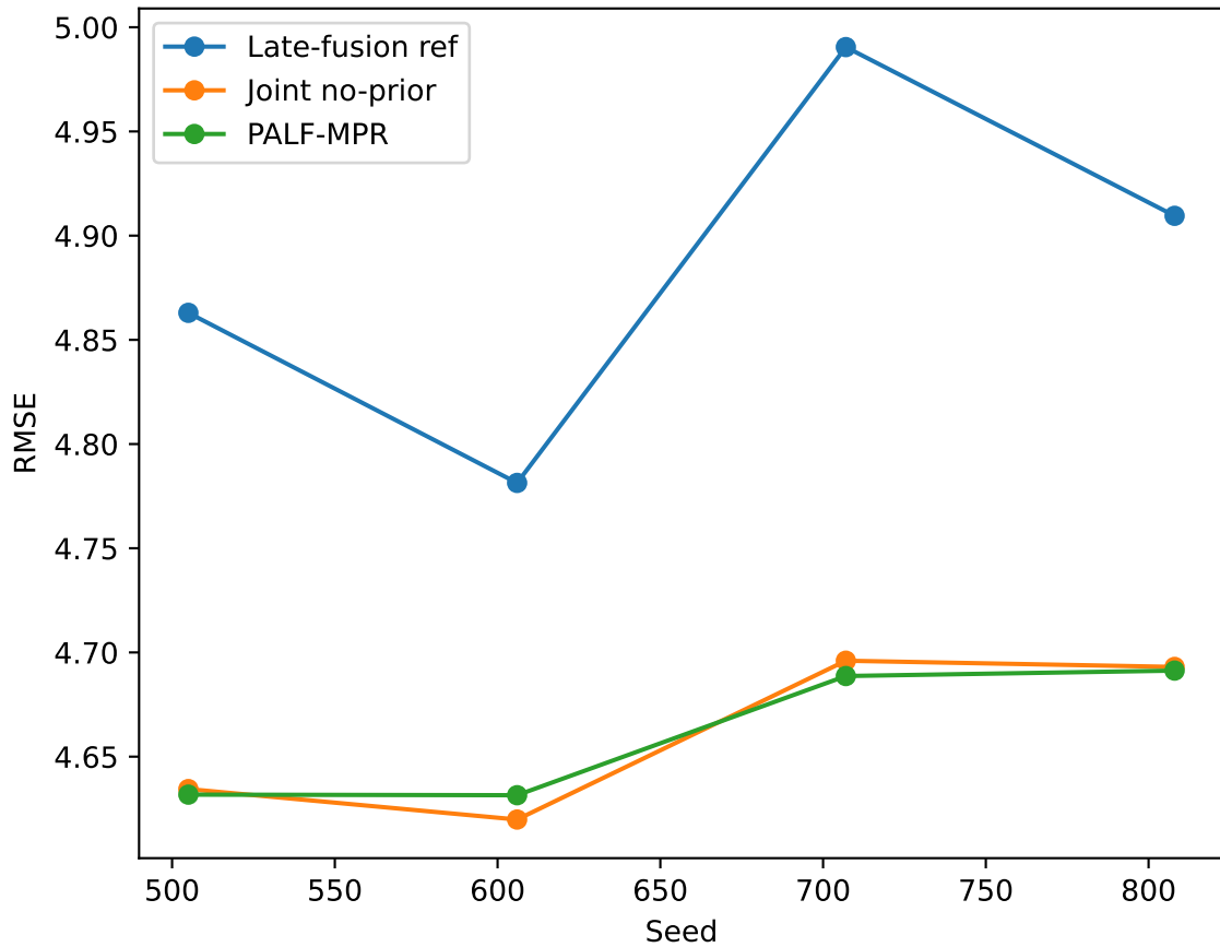
Fluid Intelligence: RMSE
