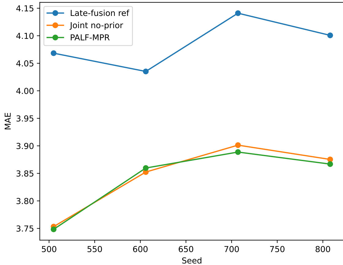
Fluid Intelligence: MAE
