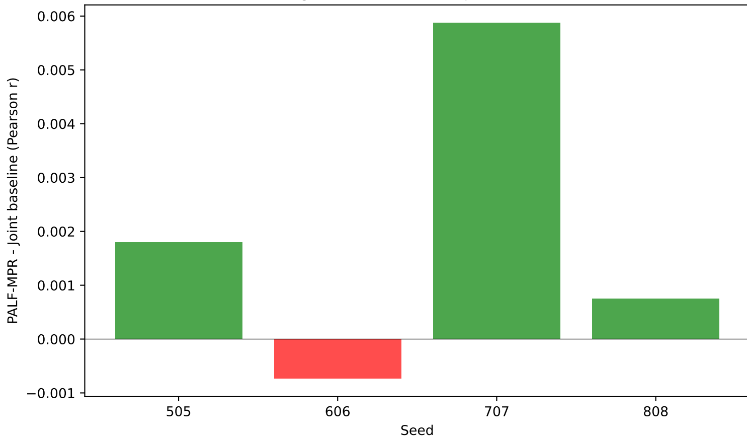
Fluid Intelligence: PALF-MPR vs Joint Baseline Delta
