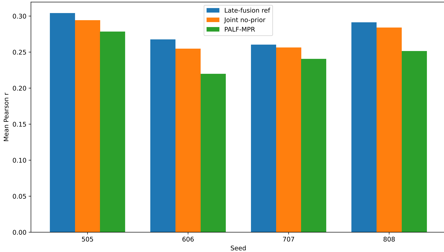
Working Memory: Three-Model Comparison
