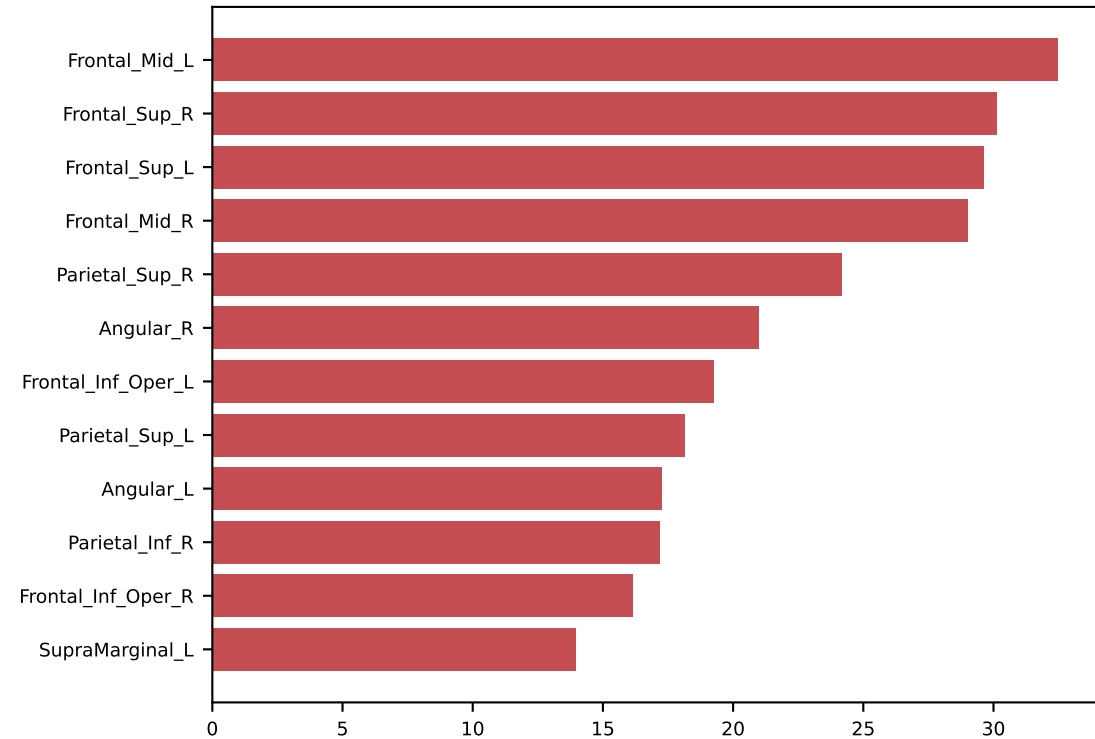
Top WM ROI importance (R-MATCHED)
