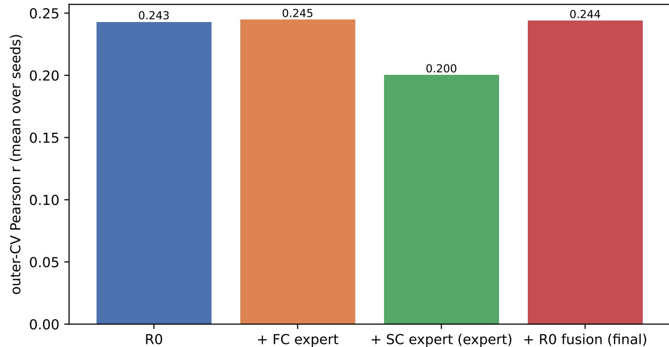
SPSEF-Ridge ablation waterfall (matched prior)
