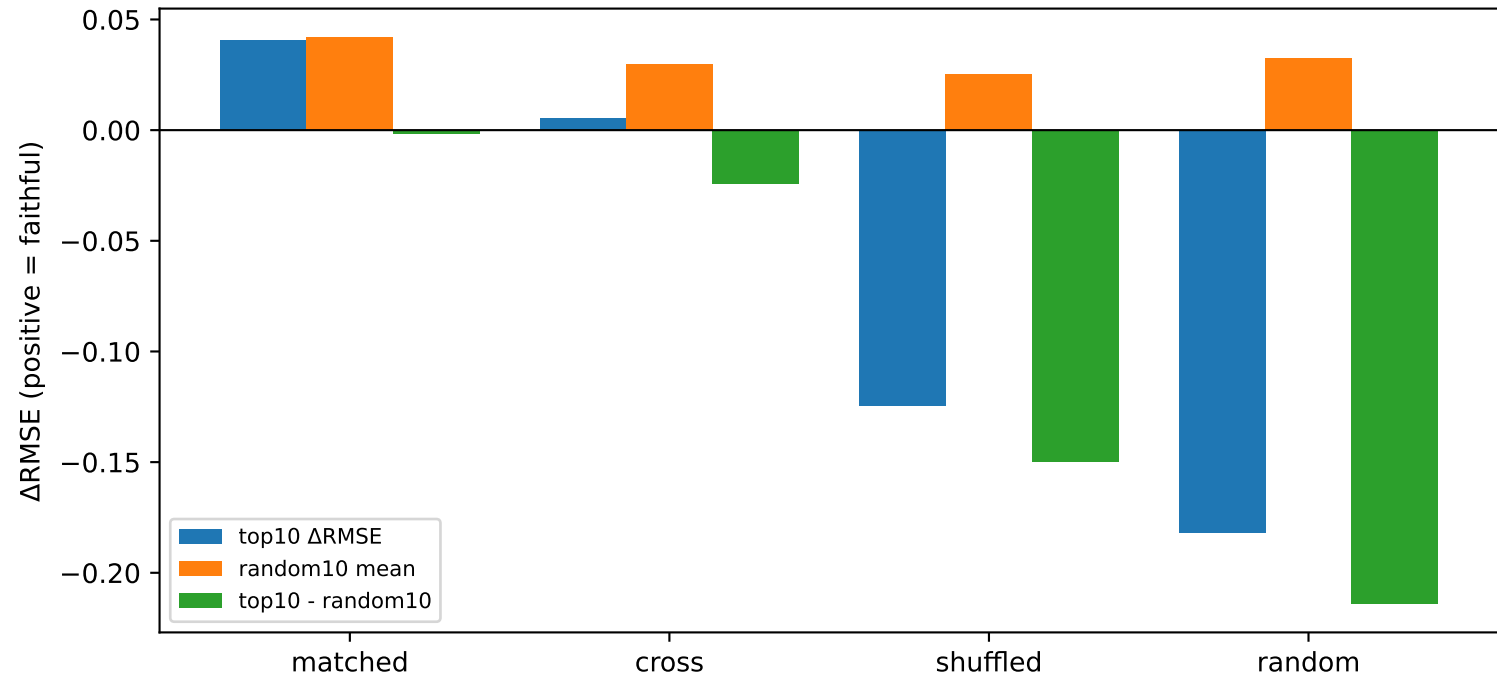
WM cross-fold faithfulness: Ridge architecture
