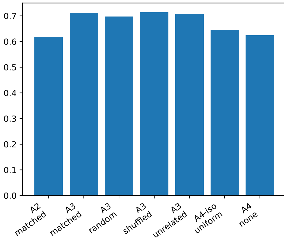
Rank stability
