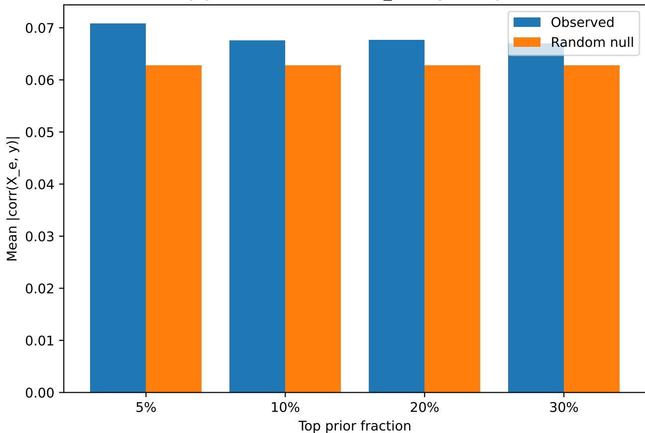
Top-prior enrichment: fluid_intelligence (prod)
