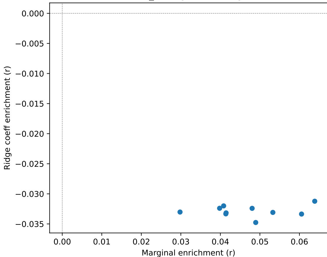
fluid_intelligence / bridge
