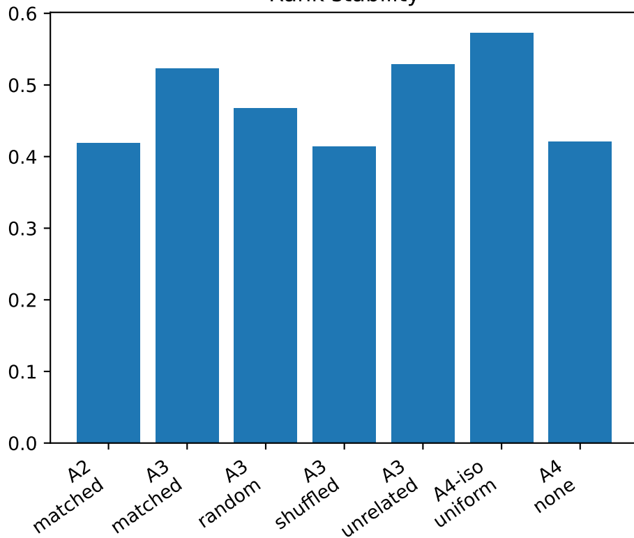
Rank stability
