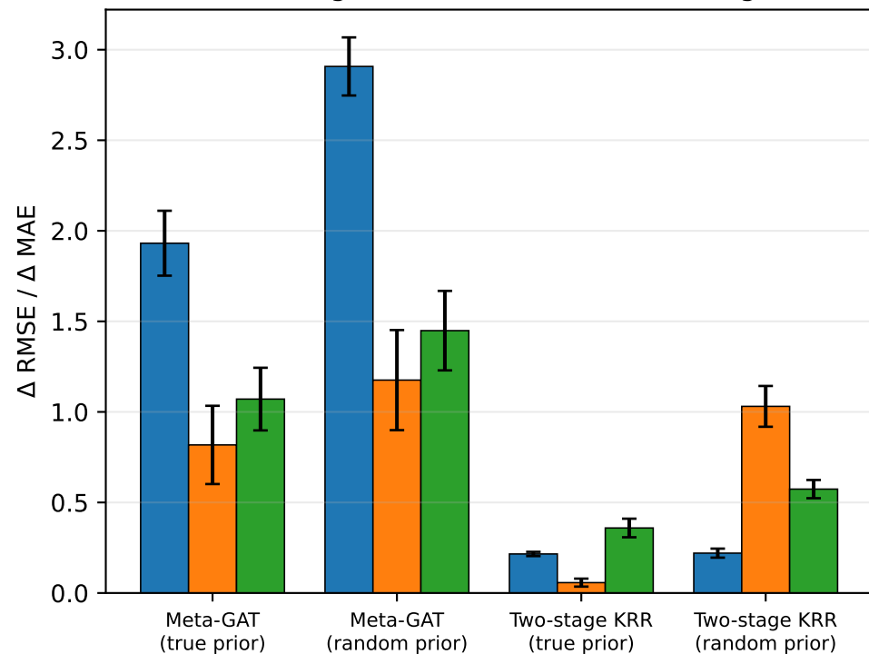
MAE degradation under ROI masking
