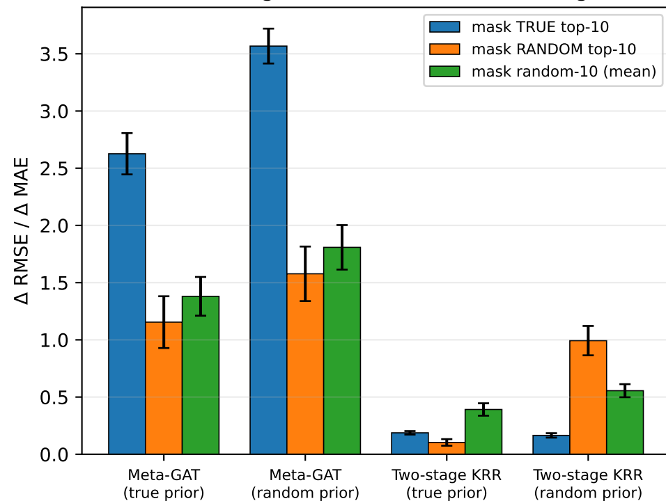
RMSE degradation under ROI masking
