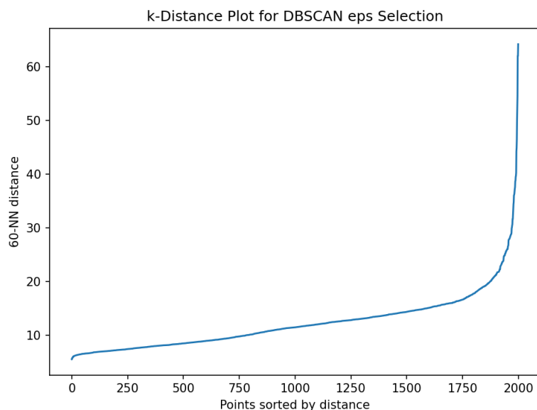
Figure 2: 60-NN distance plot used to guide the choice of \epsilon for DBSCAN.
