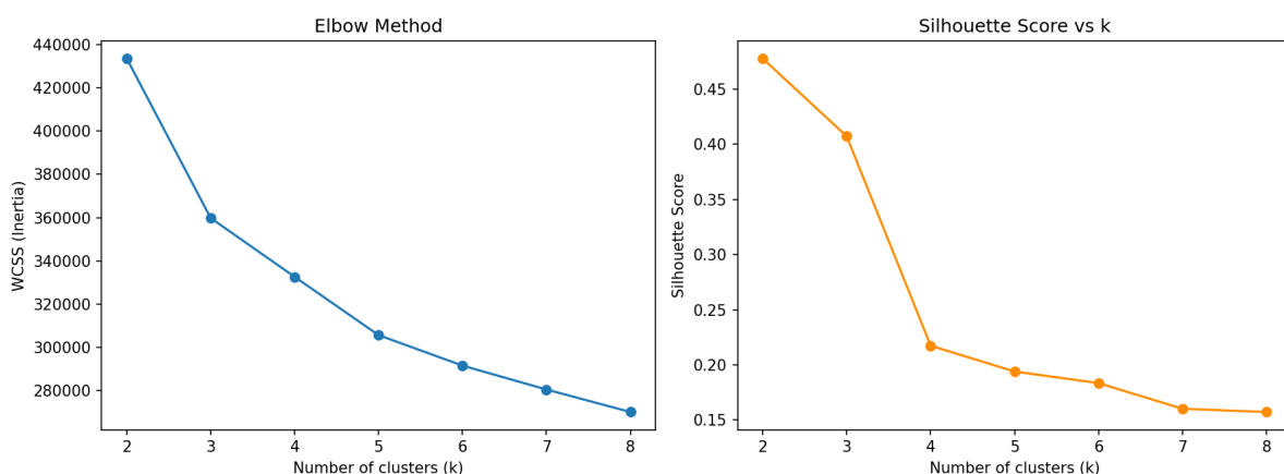
Figure 1: Elbow curve (WCSS vs k) and silhouette score vs k for K-Means.
