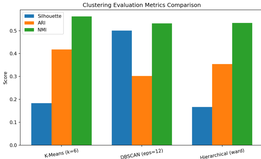
Figure 4: Silhouette, ARI and NMI compared across the three clustering algorithms.
