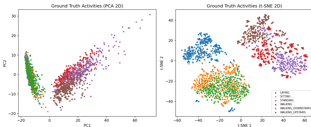
Figure 5: PCA (left) and t-SNE (right) 2D projections colored by the true activity label, for reference.
