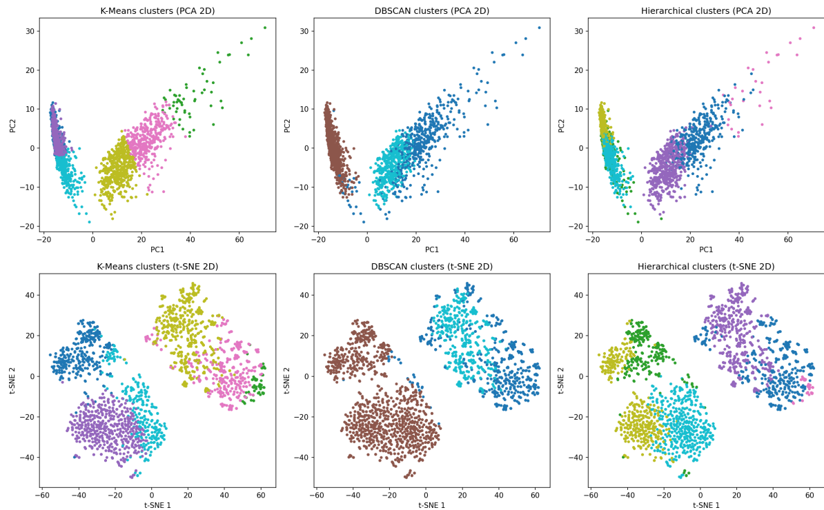
Figure 6: PCA (top row) and t-SNE (bottom row) projections colored by cluster assignment for K-Means, DBSCAN and Hierarchical (Ward) respectively.
