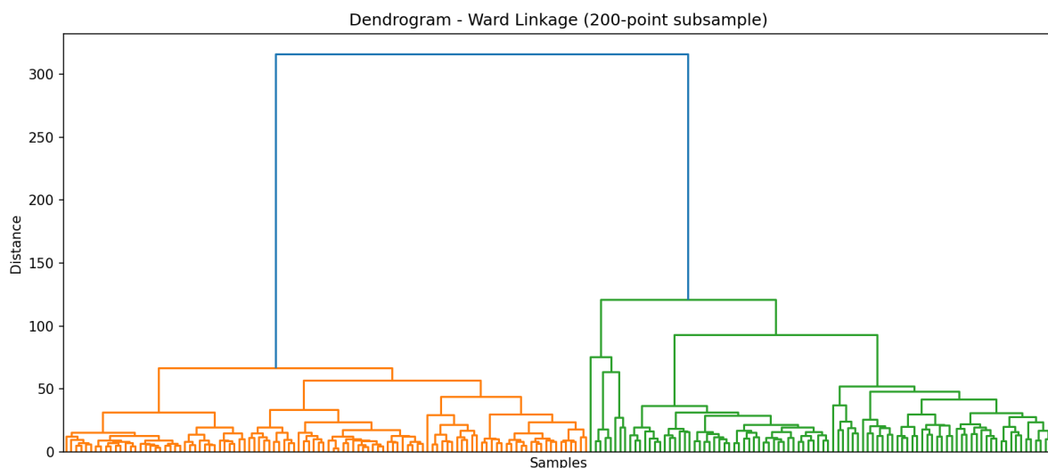
Figure 3: Dendrogram using Ward’s linkage on a 200-point subsample.
