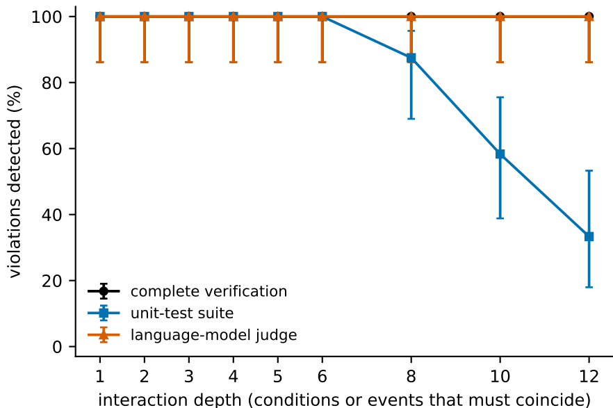
Detection of seeded violations by interaction depth
