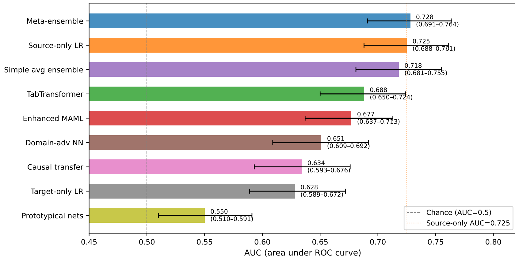
Figure 2. Model discrimination: AUC with 95% bootstrap confidence intervals Virginia hold-out test set (n=5,781; outcome prevalence 25.6%)
