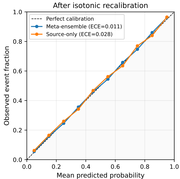
Figure 4. Reliability curves (calibration) Virginia hold-out test set (n=5,781)
