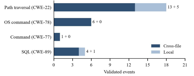
Fig. 3. Validated events by vulnerability class and scope.
