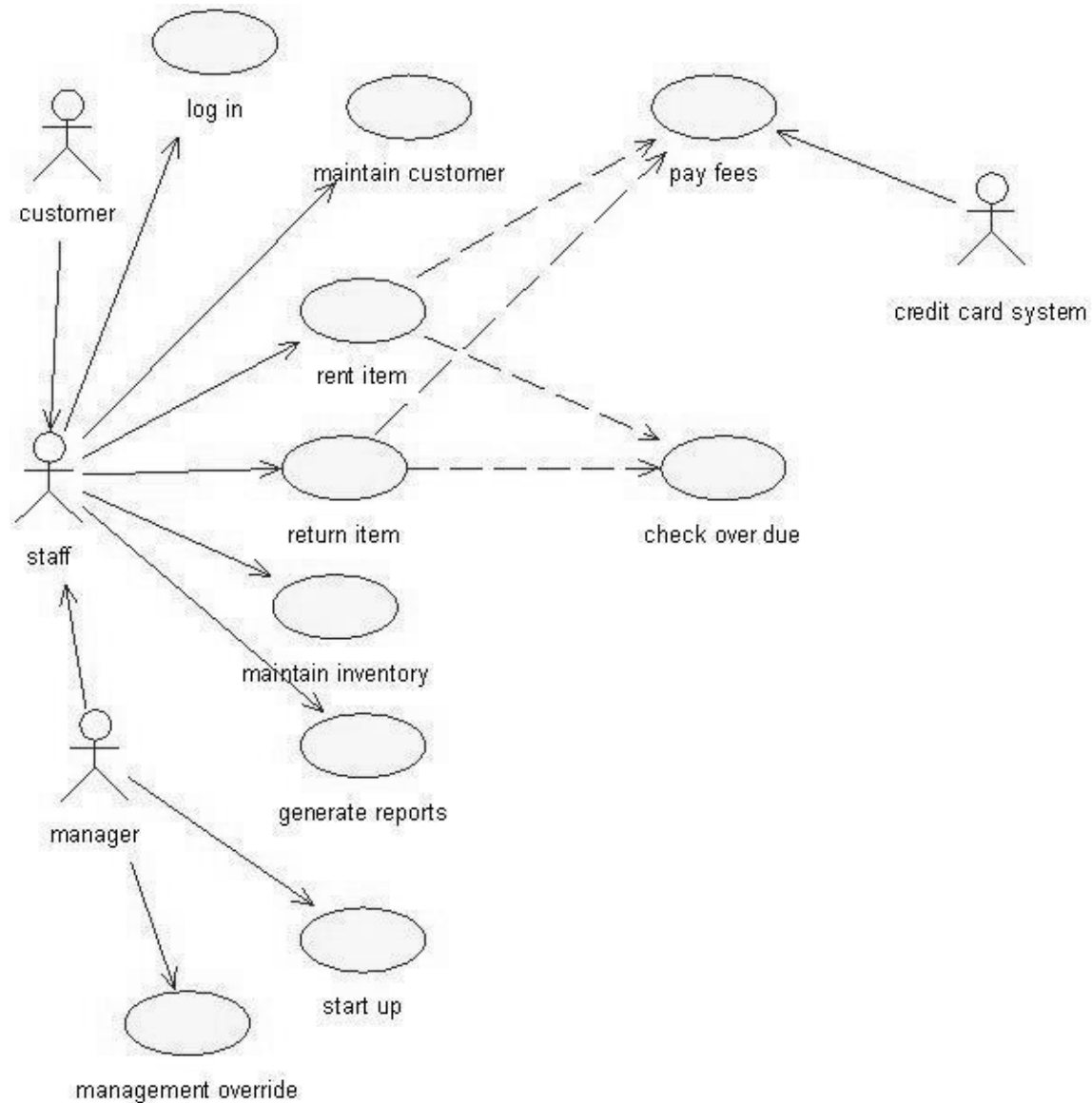
USE-CASE DIAGRAM FOR E-BOOK SYSTEM
