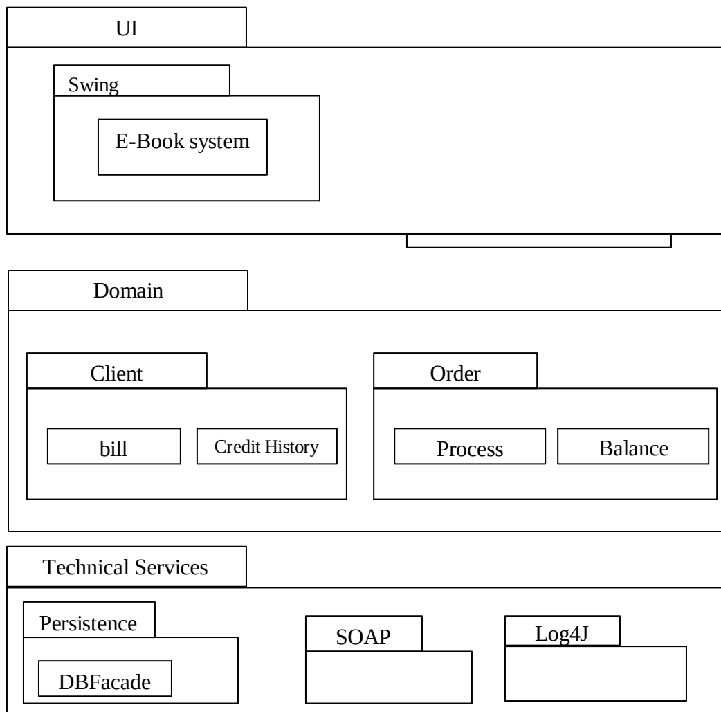
PARTIAL LAYERD LOGICAL ARCHITECTURE DIAGRAM
