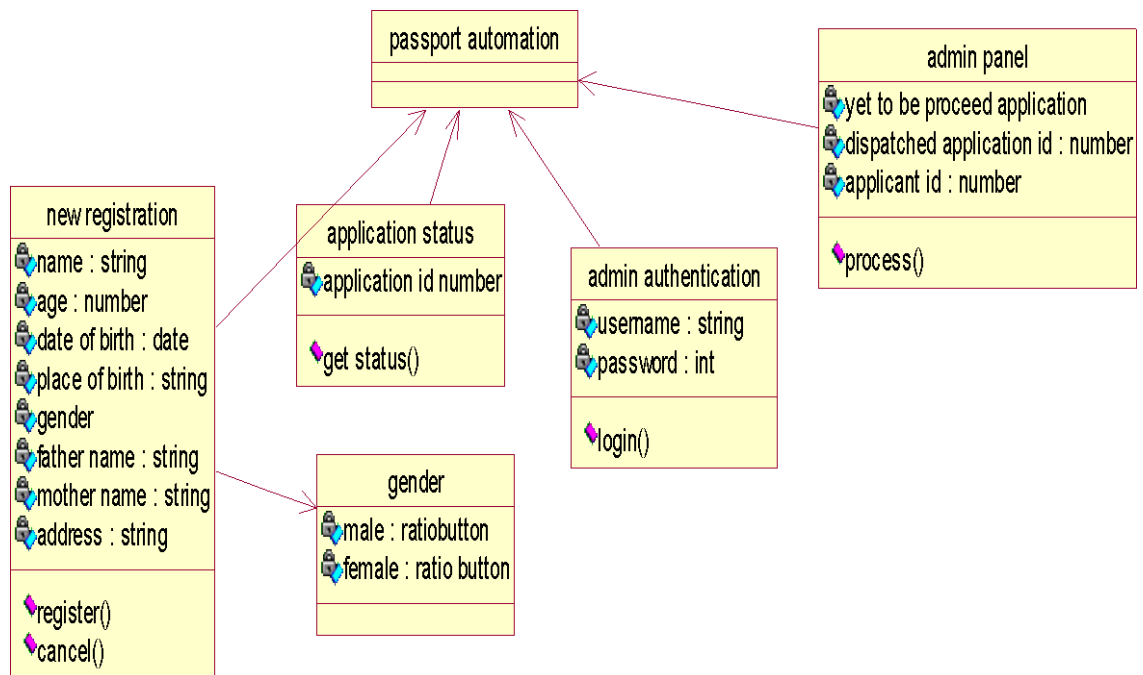
CLASS DIAGRAM FOR PASSPORT AUTOMATION SYSTEM
