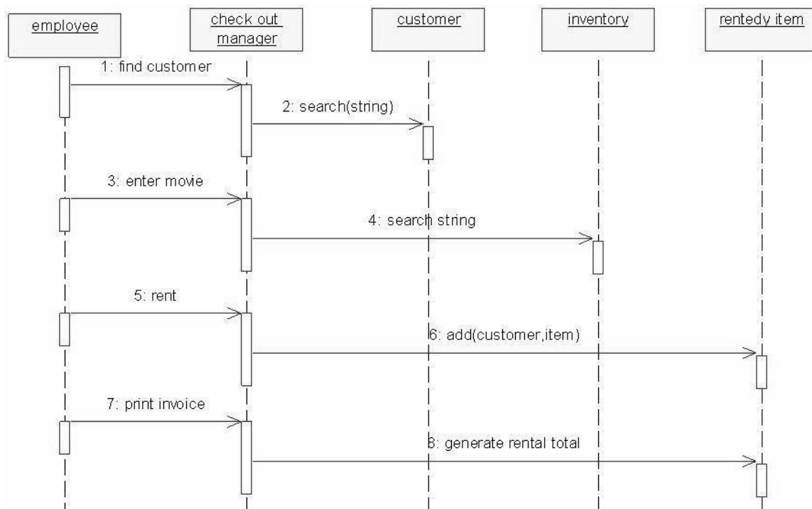
SEQUENCE DIAGRAM
