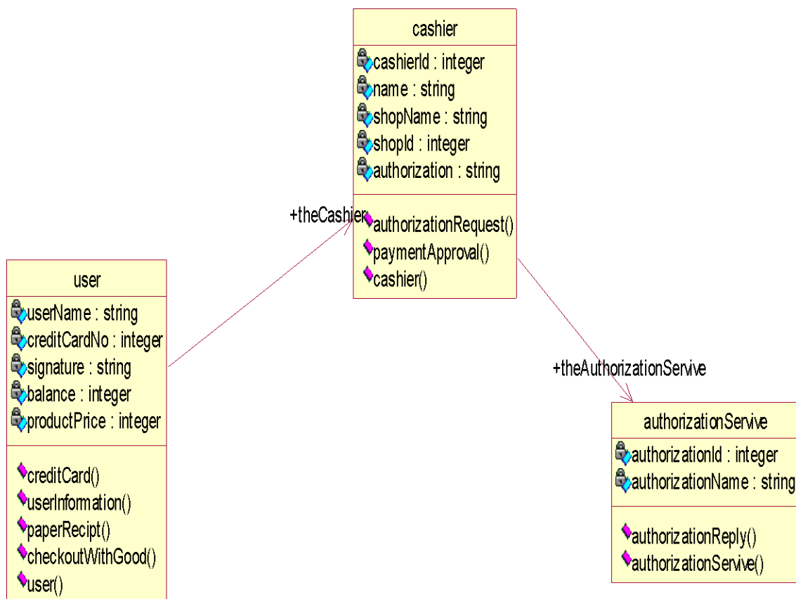
CLASS DIAGRAM
