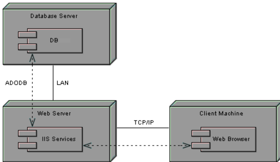
COMPONENT DIAGRAM
