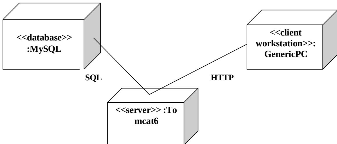
DEPLOYMENT DIAGRAM
