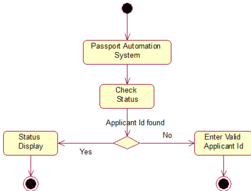
ACTIVITY DIAGRAM FOR CHECKING STATUS
