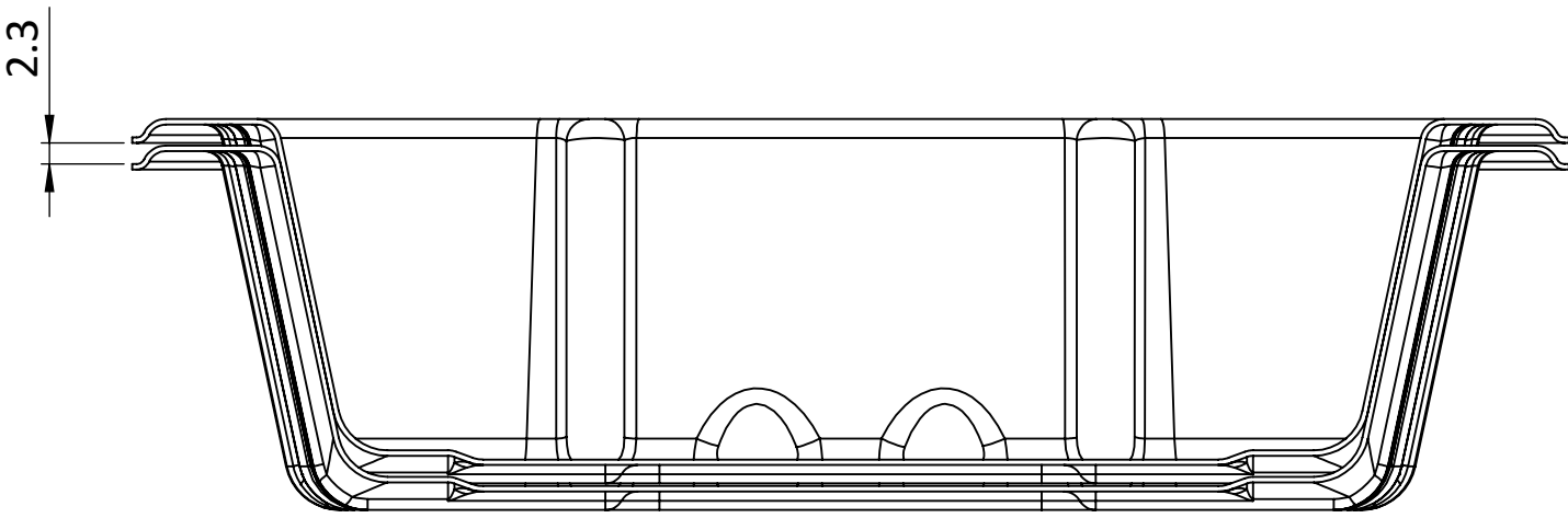
SECTION VIEW - (A - A STACKING)
