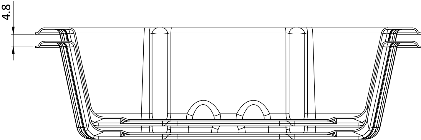
SECTION VIEW - (A - B STACKING)
